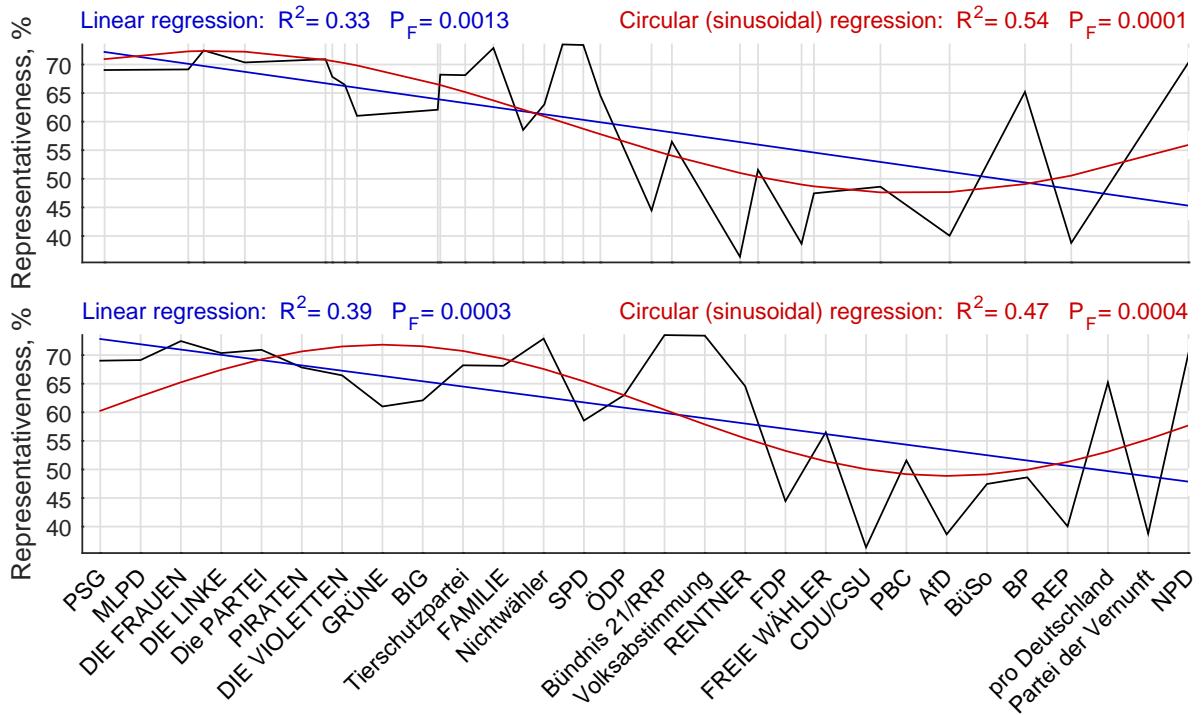
Figure 4: Principal component analysis solution. (1) Triangle of party profile correlations (in %), for the party ordering found. (2) The representativeness curve of the parties and its regression for this party ordering with taking into account the distance between neighboring parties (visualized by vertical grid lines with variable distances). (3) The representativeness curve of the parties and its regression for this party ordering without taking into account the distance between neighboring parties (visualized by vertical grid lines with equal distances).
