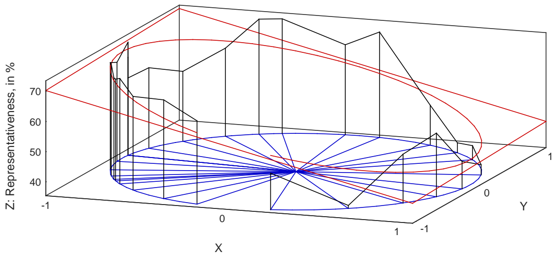
Figure 5: Traveling salesman problem solution. (1) The parties are ordered to minimize the total distance between neighboring party profiles. The distances are proportional to arc lengths (angles). The circumference is broken at the link with the largest distance between party profiles. (2) Circular regression model to fit a sinusoidal to the party representativeness curve
