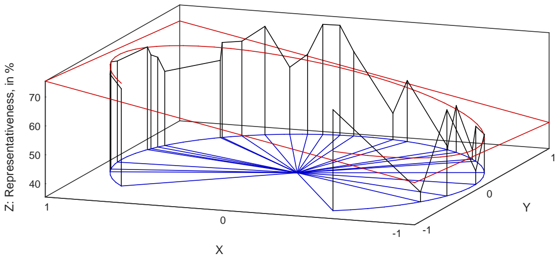
Figure 3: Principal component analysis solution. (1) Eigenvector plot for the correlation matrix of the party profiles; to visualize the left-right orientation, the direction of the first axis is reversed. Distances between party profiles are proportional to the angles between the party vectors. (2) Circular regression model to fit a sinusoidal to the party representativeness curve. The circumference is broken at the link with the largest distance between party profiles.
