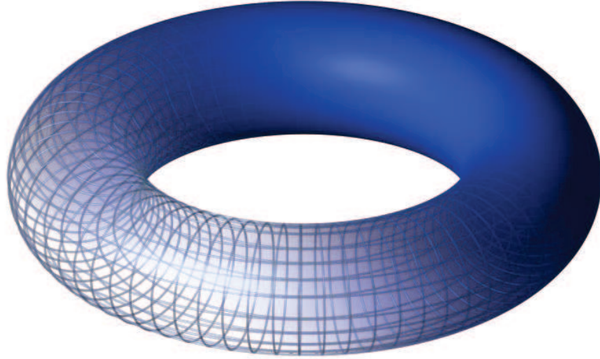
Figure 9: Torus (a bagel-like body) whose form illustrates the spatial location of party policy vectors along the circular axis with minor deviations
